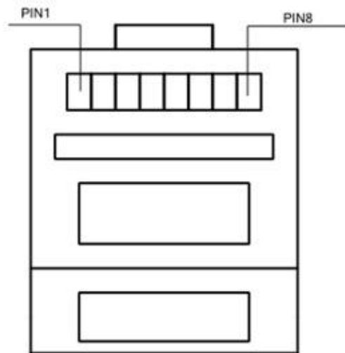
RJ45 connector, pin side
